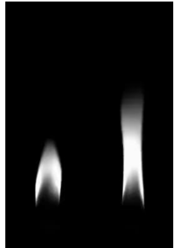
anti-phase synchronisation
